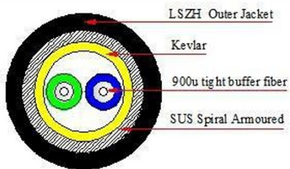
cable structure
